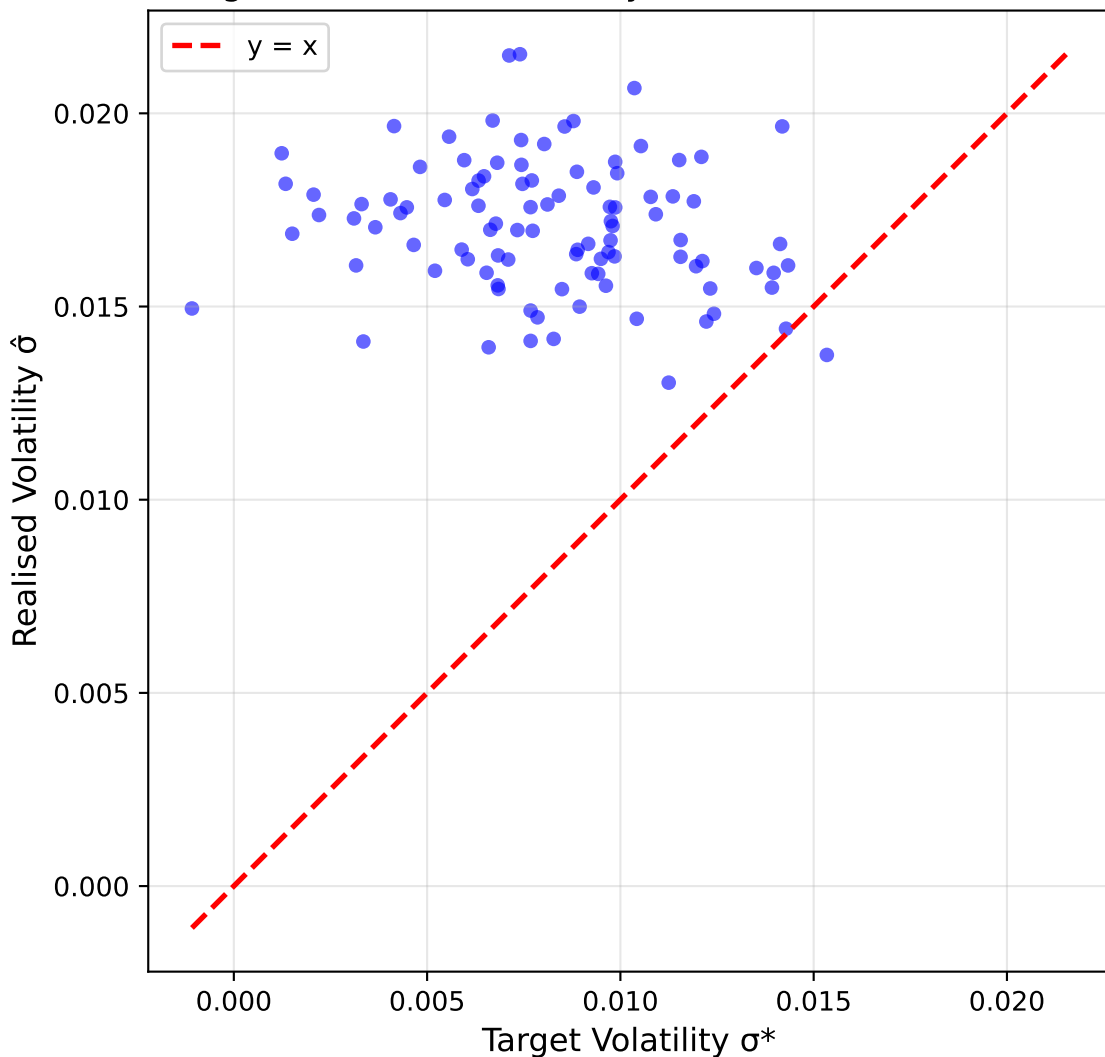
Target vs Realised Volatility ( r=-0.184 , MAE=0.0090 )
